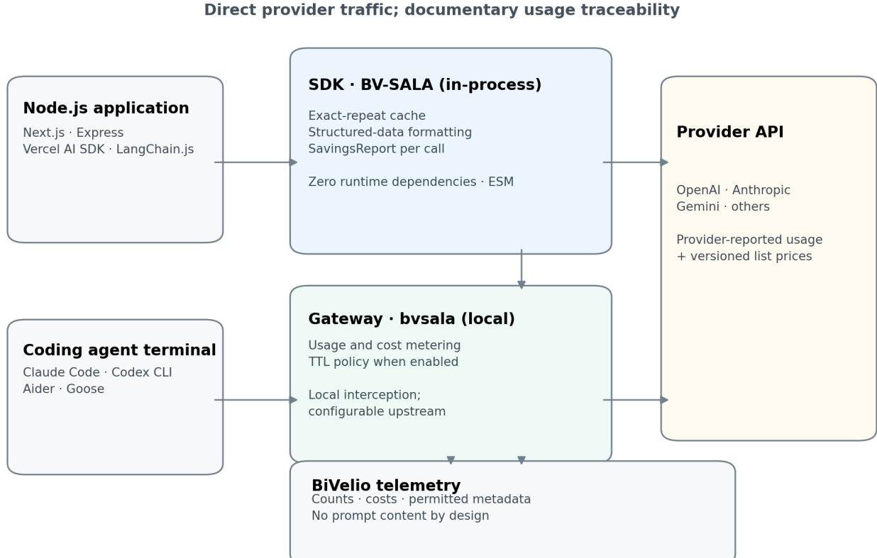
Figure 1. Deployment architecture. The SDK operates in process and the gateway locally on the configured provider path. Costs are computed from provider-reported usage and versioned list prices. Telemetry comprises counts, costs, and permitted metadata rather than prompt content by design; deployment configuration still requires review.
