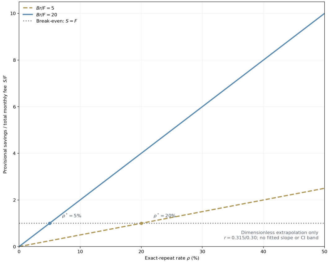
Figure 3. Provisional, dimensionless extrapolation only. S/F = (B \cdot r/F)\rho , with r = 0.315/0.30 from one OpenAI operating point. Lines for B \cdot r/F = 5 and 20 intersect S = F at \rho^* = 20\% and 5\% , respectively. This is not a regression, a measured dose-response relationship, or a forecast for other workloads.
