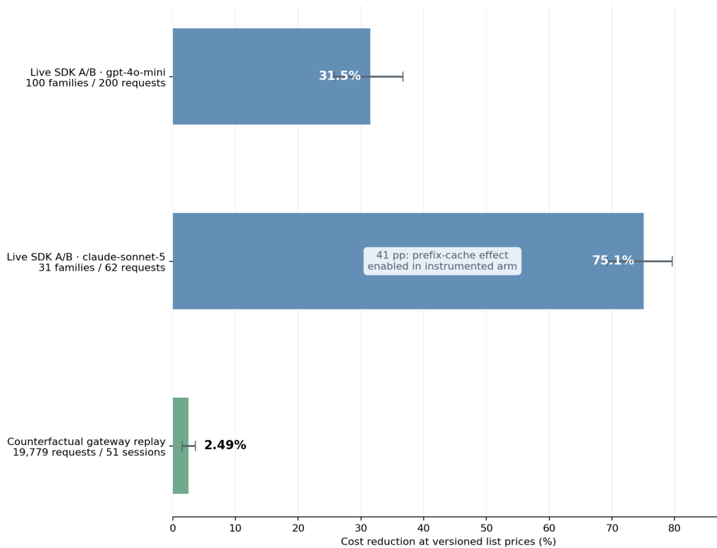
Figure 2. Cost reductions at versioned list prices with 95% cluster-bootstrap intervals. OpenAI and Anthropic are live SDK double-runs; the gateway result is a counterfactual replay, not a live double-run. In the Anthropic experiment, approximately 41 percentage points are a prefix-cache effect enabled by cache_control in the instrumented arm. Error bars show the reported intervals.
